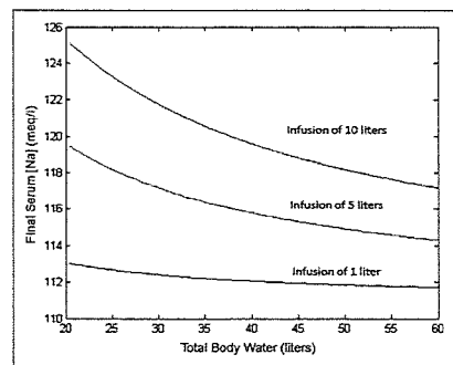
Figure 4. Effect of varying body water estimates on the change in serum sodium concentration of a patient with initial serum sodium concentration ([Na]) of 111 mEq/L infused with various volumes of 0.154 mol/L saline. Calculations from formula 7 (Table 3).
