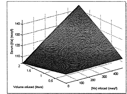
Figure 3. Serum sodium concentration changes ([Na]) after infusion of 1.75 L of saline with varying sodium concentration in a patient with initial body water of 26 L and initial [Na] of 111 mEq/L. The changes in [Na] were computed by formula 7 of this report.
