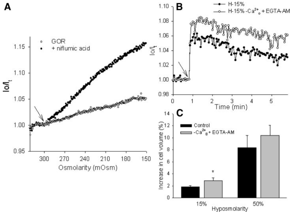
Fig. 2. Ca^{2+} dependence and effect of niflumic acid on cell volume changes of C6 cells exposed to SOR or GOR. Estimation and expression of relative cell volume change ( I_0/I ) as in Fig. 1. A : a representative experiment of cell volume changes elicited by GOR in the presence (●) or absence (○) of 600 \mu M niflumic acid. Niflumic acid was present throughout the experiment. B : representative traces of cell volume changes elicited by 15% SOR in the presence or absence of intracellular Ca^{2+} . Cells were superfused with isosmotic medium, and then (arrow) medium was made -15% hyposmotic (●) by addition of distilled water. Cell volume changes were followed 10 min after hyposmotic stimulus. ○, Cells were preloaded with 50 \mu M EGTA-AM 30 min before the experiment, and isosmotic medium was made nominally Ca^{2+} -free by addition of 0.5 mM EGTA. C : effect of Ca^{2+} -free conditions (as described in B ) on cell volume increase attained during GOR. Bars represent cell volume increase (% over isosmotic condition) reached at H-15% and H-50%. Solid bars, volume changes in the presence of Ca^{2+} ; shaded bars, volume changes in cells in Ca^{2+} -free conditions as in B . Results are means \pm SE; n = 4 . * P < 0.05 vs. control.
