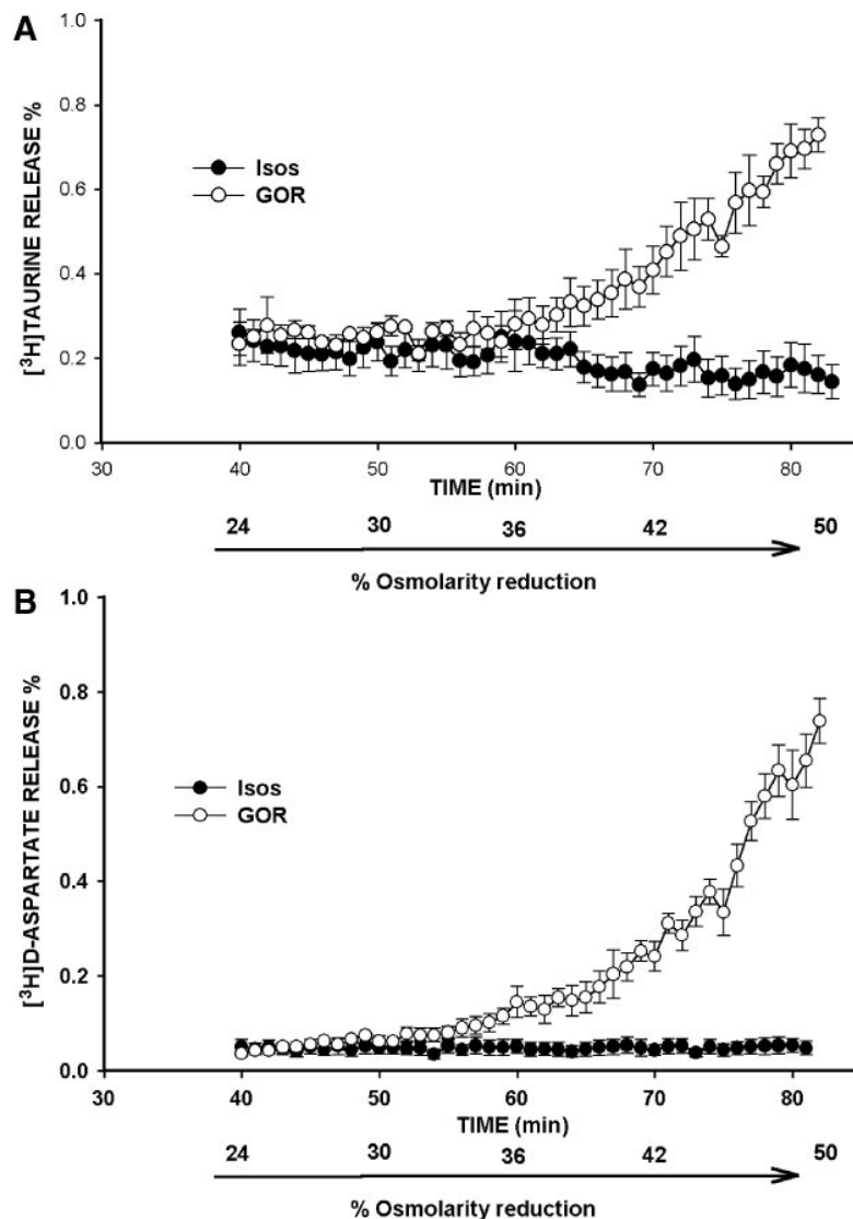
Fig. 10. Amino acid release from C6 glioma cells elicited by GOR. Cells were preloaded with [ ^3\text{H} ]taurine (A) or D-[ ^3\text{H} ]aspartate (B) as described in MATERIALS AND METHODS. After a basal collection period of 6 min with isosmotic medium, the external osmolarity was decreased at a rate of 1.8 mosM/min and superfusion continued until -50\% reduction in osmolarity was achieved (final osmolarity 150 mosM). Controls were continuously superfused with isosmotic medium. Fractions were collected every minute from minutes 1 to 82, but because no difference was observed during the first 50 min, the points show only the time course of efflux from minute 40 to the end. Data are expressed as efflux rate constants ( \text{min}^{-1} ) and are means \pm SE of 6 experiments.
