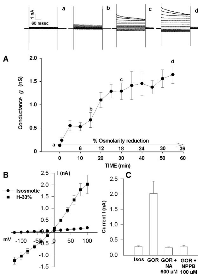
Fig. 5. A: \text{Cl}^- conductance elicited by GOR in intracellular \text{Ca}^{2+} -free conditions. The pipette was filled with 140 mM CsCl, the holding potential was -70 mV ( n = 6 ). Insets a–d show the current activation at the osmolarity indicated by letters in the plot. B: I - V curves in cells in isosmotic medium and at H-33%. C: effect of the \text{Cl}^- channel blockers niflumic acid (NA) and 5-nitro-2-(3-phenylpropylamino)benzoic acid (NPPB) on the GOR-elicited \text{Cl}^- current. The blockers were present in the solutions used to generate the media with gradually decreased osmolarities. Bars represent means \pm SE ( n = 4 ) of the current measured at +100 mV.
