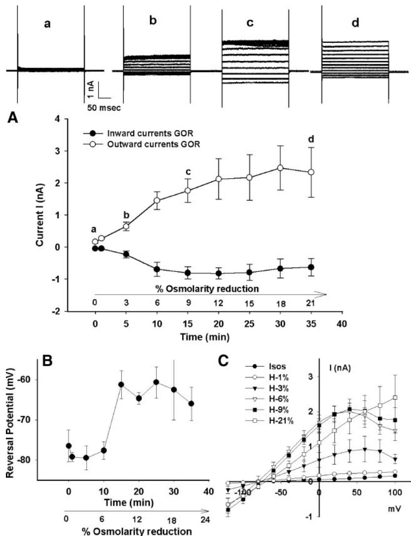
Fig. 6. Whole cell currents activated by GOR in the presence of intracellular \text{Ca}^{2+} . A: membrane currents measured as in Fig. 3 but with 200 nM \text{Ca}^{2+} in the patch pipette ( n = 6 ). Insets a–d show the activation of currents at the time and osmolarity marked by letters in the plot. B: change in the membrane potential (initial -78 \pm 3 mV) through the effect of GOR. C: I - V relationship in cells in isosmotic medium and at osmolarity reductions as indicated.
