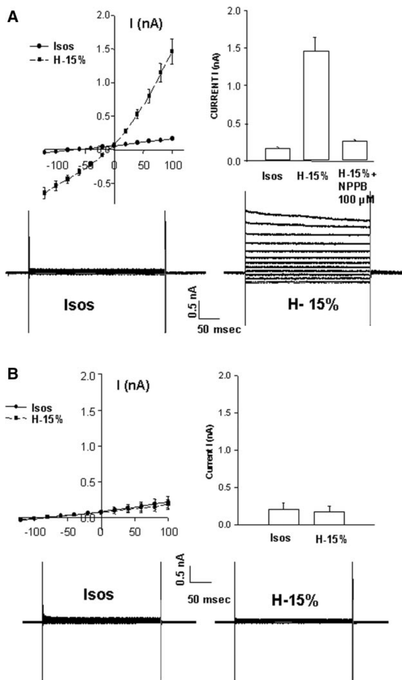
Fig. 8. K + and Cl - currents activated by a sudden decrease in osmolality of 15% in Ca 2+ -free conditions. Cl - (A) and K + (B) currents were measured as in Fig. 3, with ionic replacements and effect of Cl channel blockers as in Figs. 4 and 5; n = 6 .
