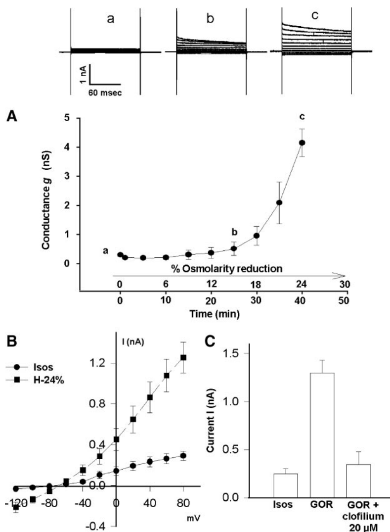
Fig. 4. K + conductance ( g ) elicited by GOR in intracellular Ca 2+ -free conditions. The pipette was filled with 130 mM K-aspartate. The holding potential was -70 mV ( n = 6 ). A: insets a–c show the currents obtained at the osmolarity indicated by letters in the plot. B: I - V relationships for K + currents ( n = 6 ) under isosmotic conditions and at H-24%. C: effect of clofilium on the GOR-elicited K + current. Bars represent means \pm SE ( n = 5 ) of the current measured at +80 mV.
